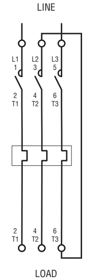
Diagram 4 - Power connection for 1-phase motors
