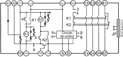
G9SA-301 (24 Vc.a./Vc.c.)
