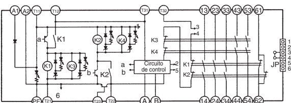
G9SA-501 (24 Vc.a./Vc.c.)
