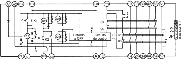
G9SA-321-T□ (24 Vc.a./Vc.c.)
