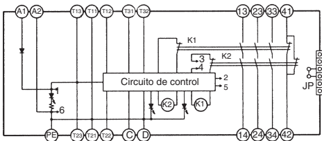
G9SA-TH301 (24 Vc.a./Vc.c.)
