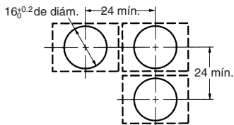
A16□-J/M16□-J rectangular (vista superior)
