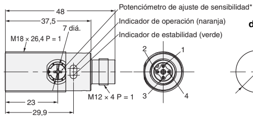
Vista frontal
