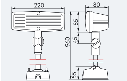
Ecolight 18-WA
