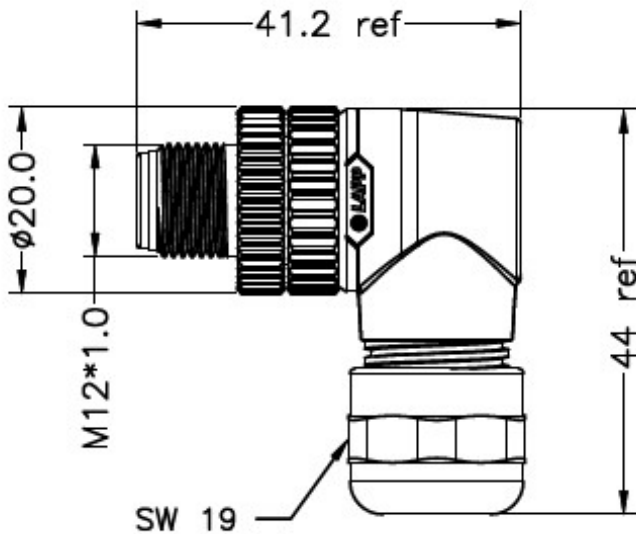
Technical drawing
