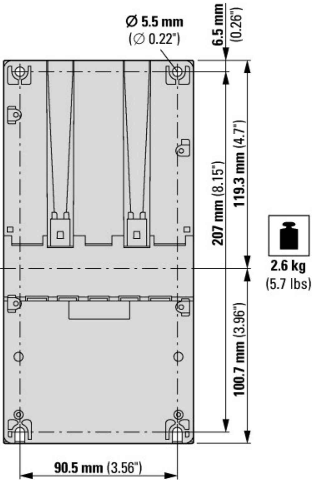
Back view
