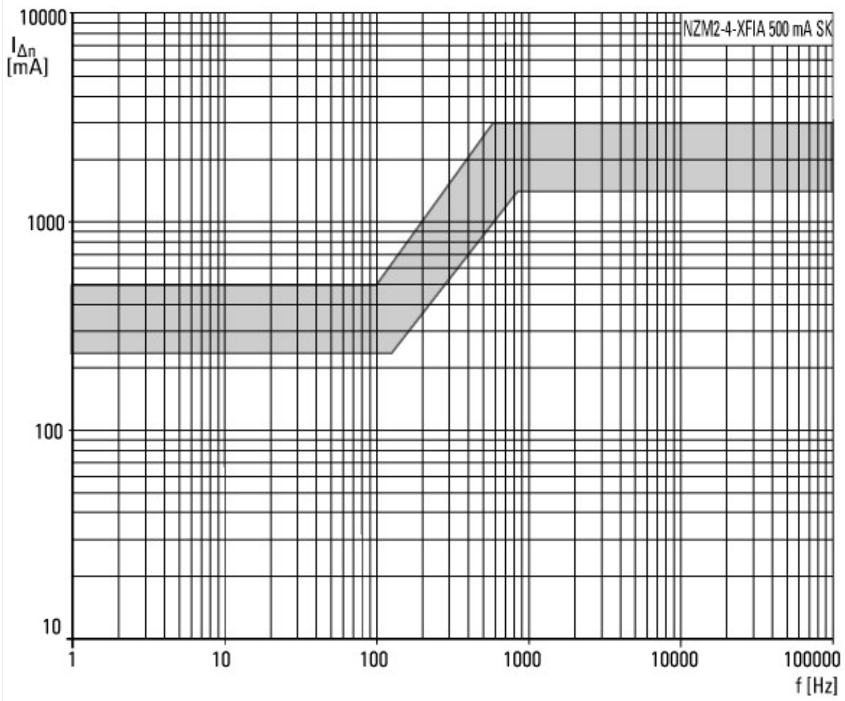
Tripping current frequency response 500 mA SK part no.
