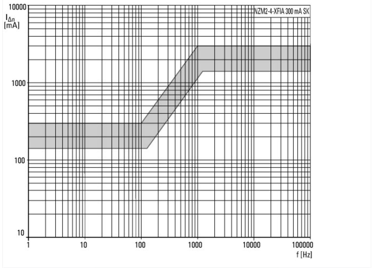
Tripping current frequency response 300 mA SK part no.
