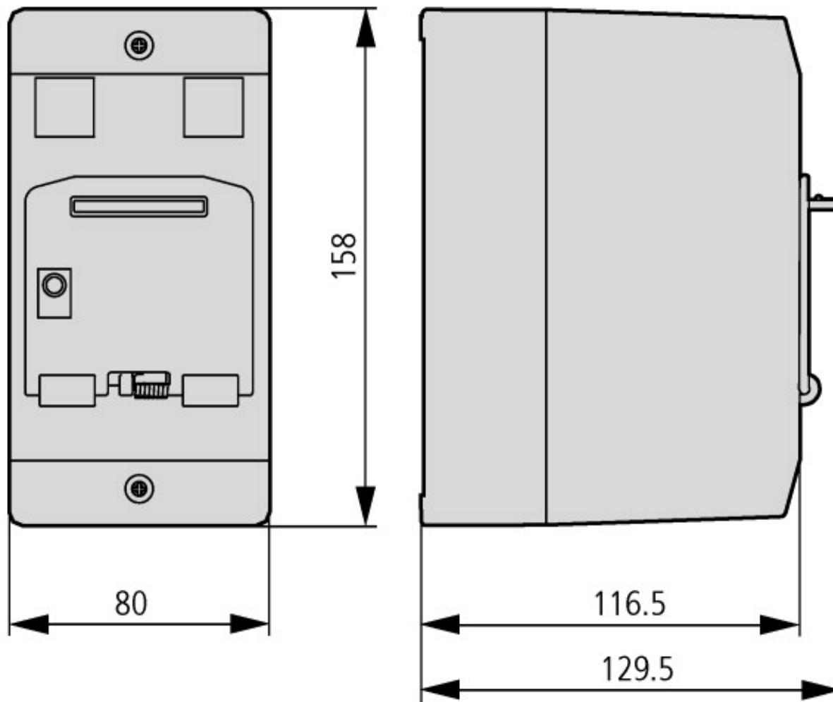
Insulated enclosure for top mounting
