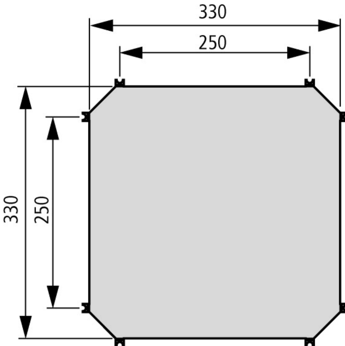
IM4-... insulated mounting plate 4 mm thick
