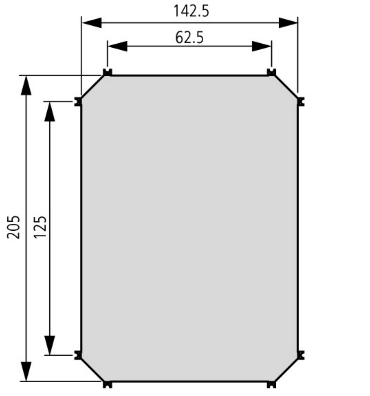
IM4-... insulated mounting plate 4 mm thick
