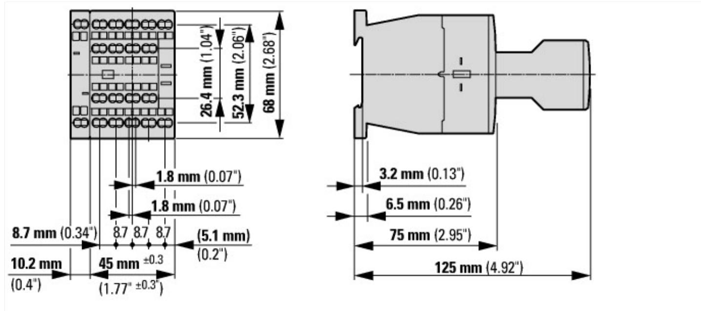
Contactor with auxiliary contact module
