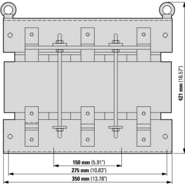
2 x Inverter
