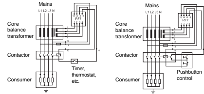
Circuit diagram with continuous contact control Circuit diagram with impulse contact control
