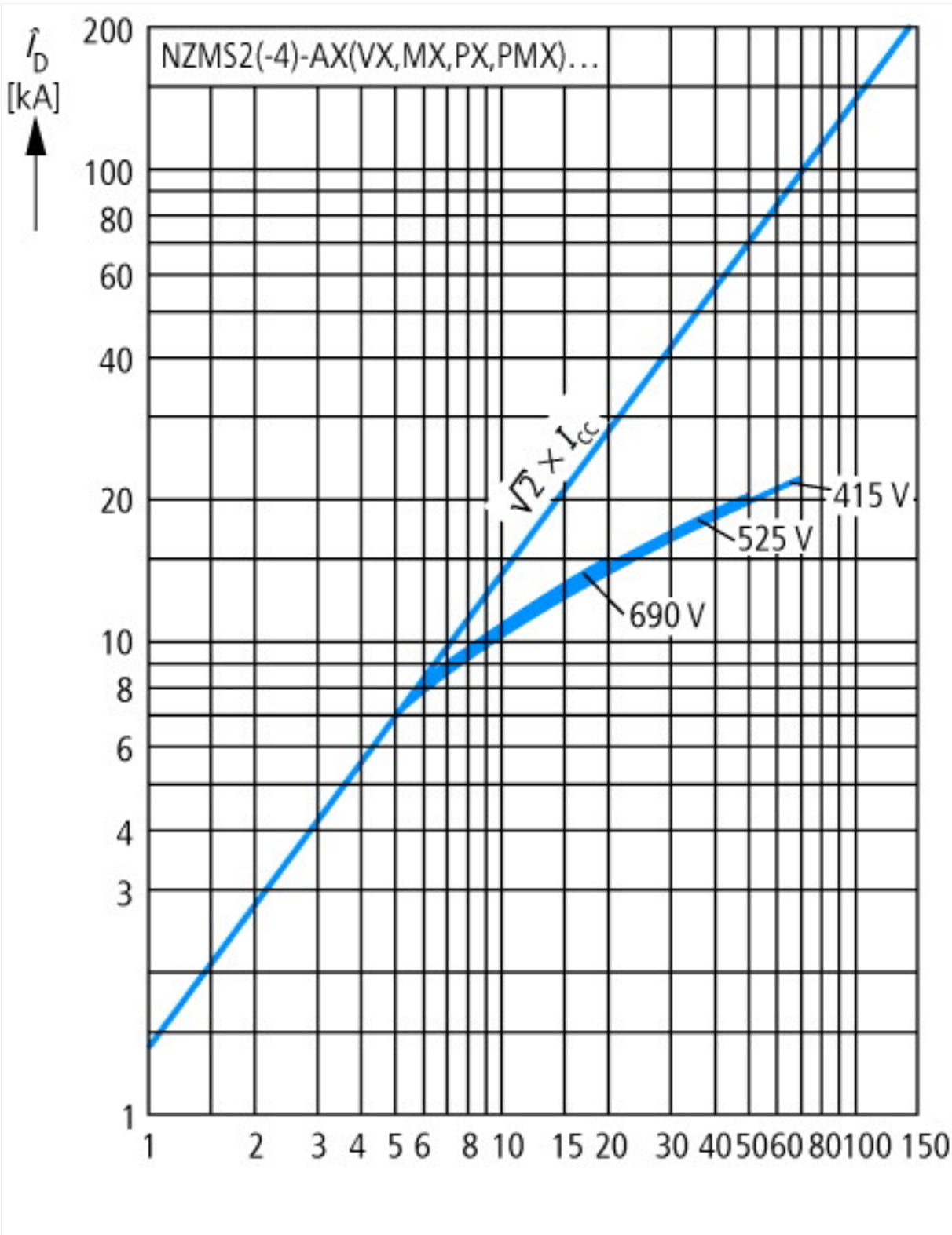
Let-through current
