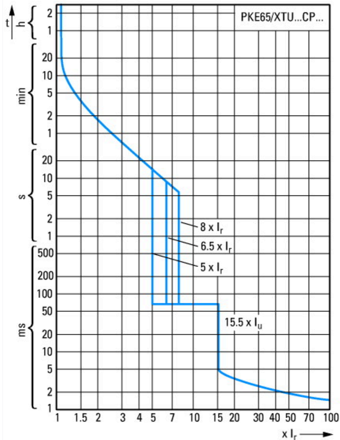
Tripping characteristics
