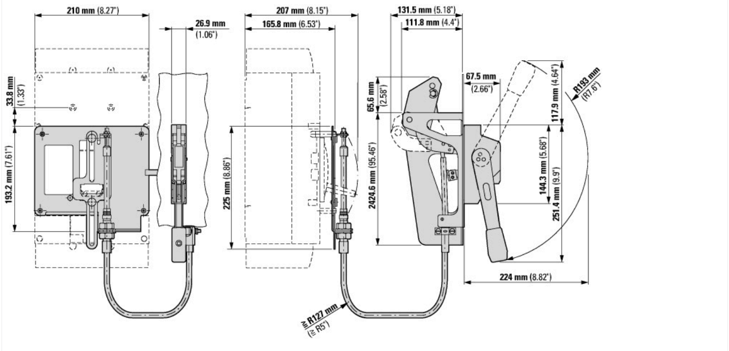
Flange mounted handle kit Type 4X 48°
