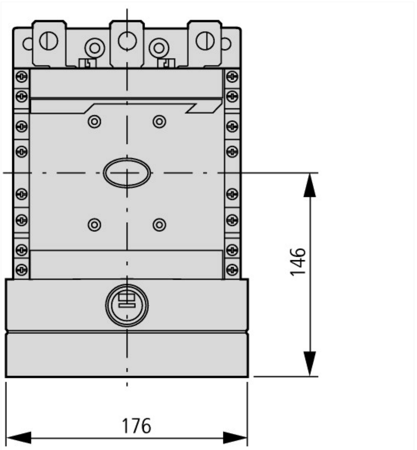
Contacteur with star-point bridge and terminal shroud for DILM500
