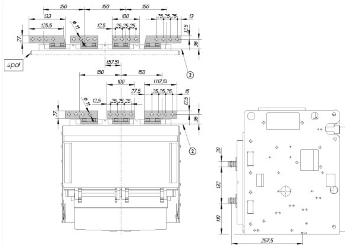
② Contact surface flange terminal
