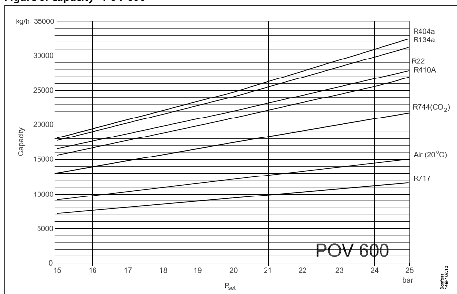
Figure 6: Capacity - POV 600
