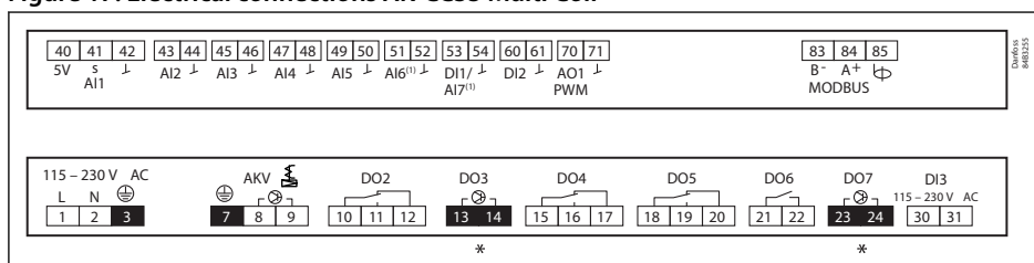
Figure 17: Electrical connections AK-CC55 Multi Coil
