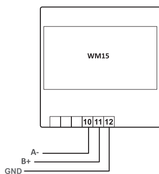
Fig. 14 Porta RS485
