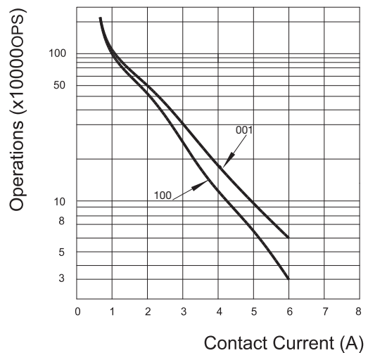
ENDURANCE CURVE
