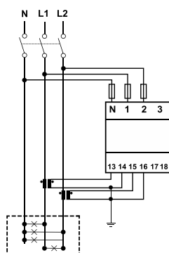
Fig. 8 Two-phase system with neutral (3-wire)
