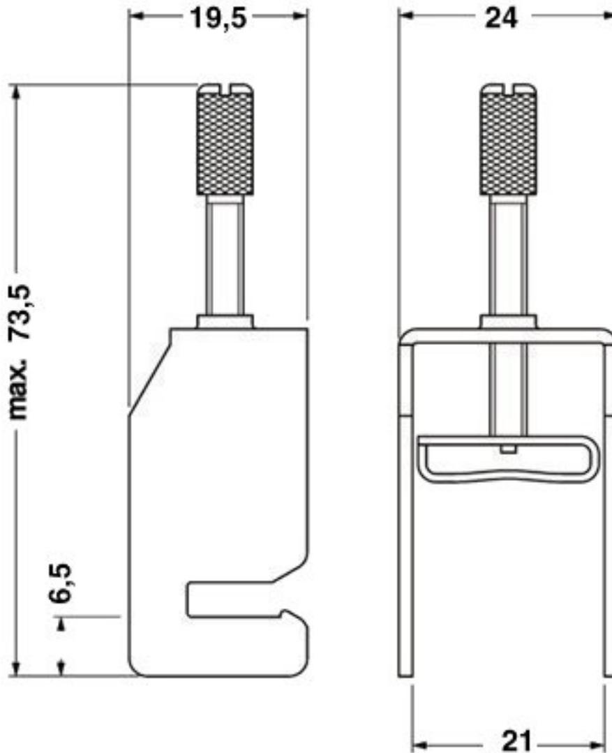
Dimensional drawing
