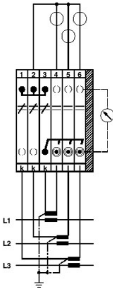
Schematic diagram
