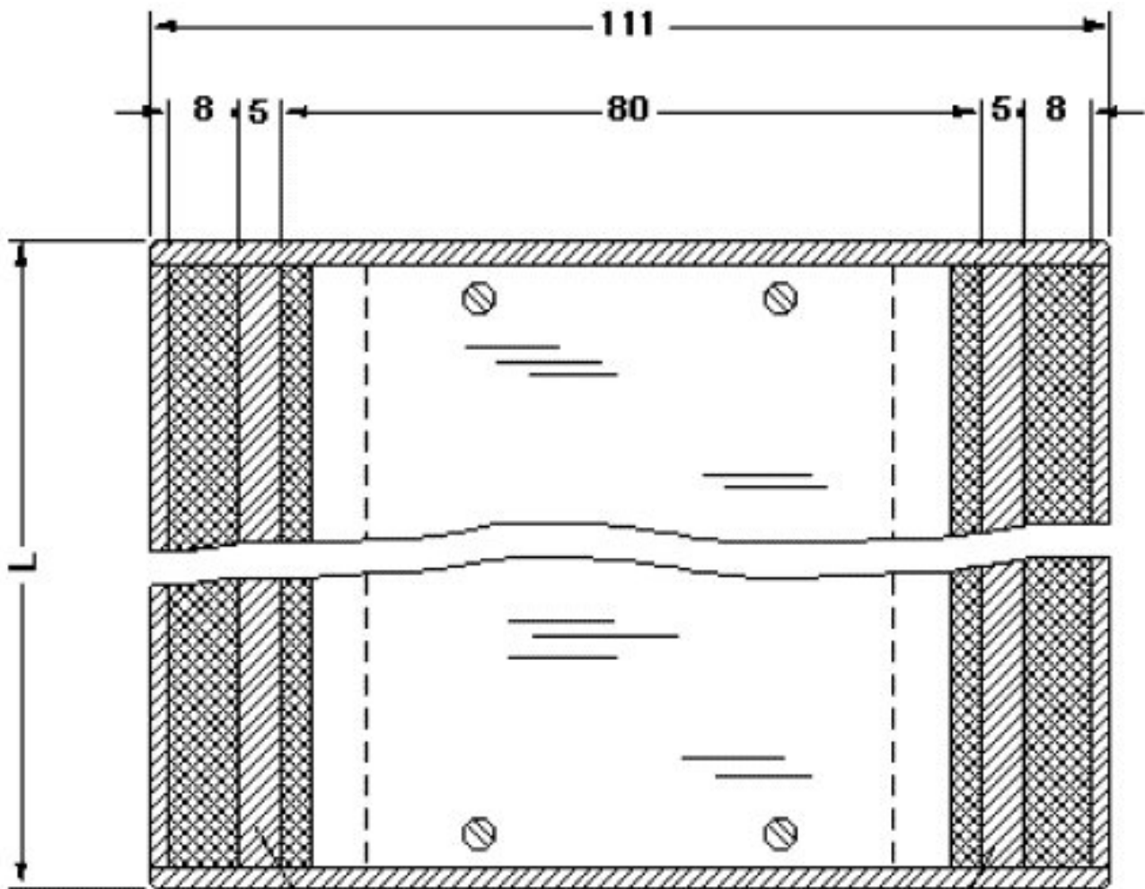
Dimensional drawing
