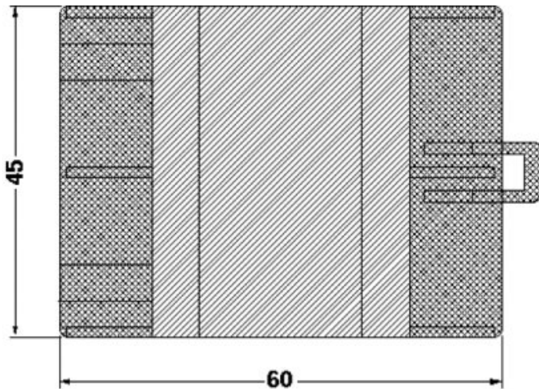
Dimensional drawing
