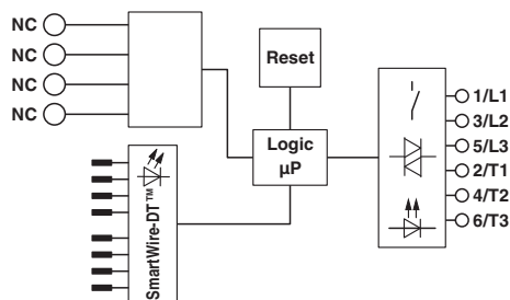
Block diagram
