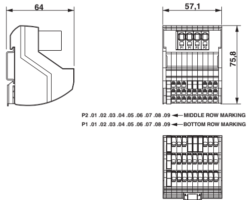
Dimensional drawing
