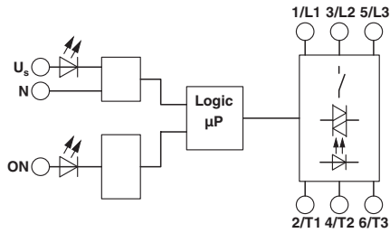
Block diagram
