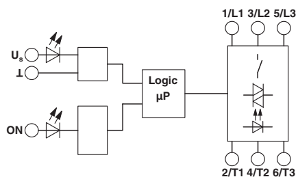
Block diagram
