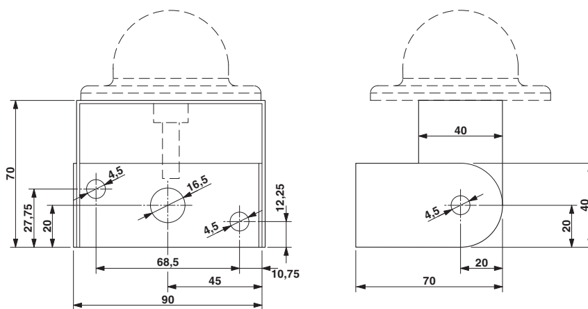
Dimensional drawing
