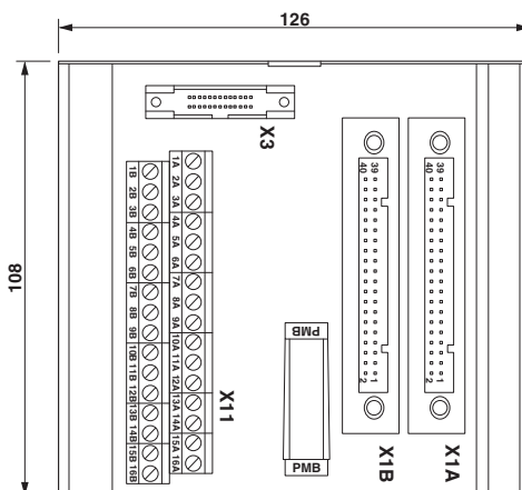
Dimensional drawing
