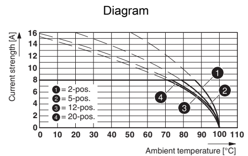
Type: FRONT-MC 1,5/...-ST-3,81 with MCV 1,5/...-G-3,81
