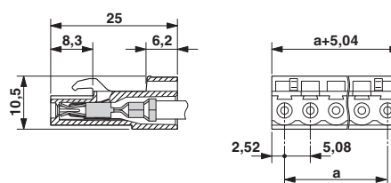
Dimensional drawing
