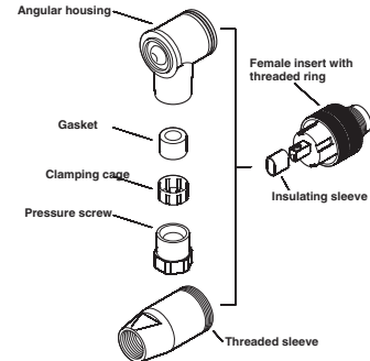
Schematic diagram
