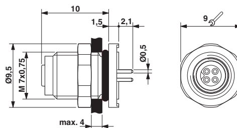
M5 flush-type socket
