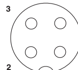
Pin assignment M12 socket, A-coded
