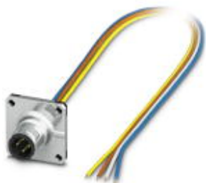
Sensor/actuator flush-type plug, 4-pos., M12, D-coded, front/square flange mounting, with 0.5 m TPE litz wire, 4 x 0.34 mm 2
