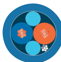
Fieldbus FOUNDATION/PROFIBUS PA, blue [961]
