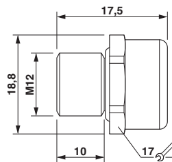
Dimensional drawing
