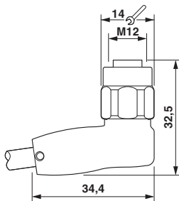
Dimensional drawing
