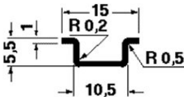
Dimensional drawing
