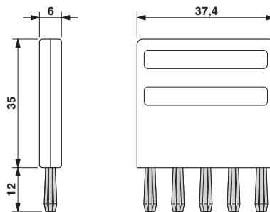
Dimensional drawing
