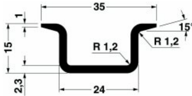
Dimensional drawing
