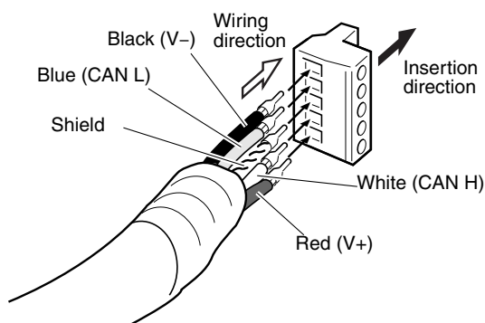
Straight Connector without Attachment Screws
