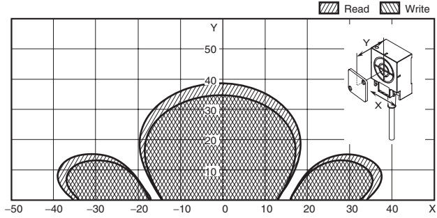
V680-H01 (mounted on non-metallic material) & V680-D1KP58HT
