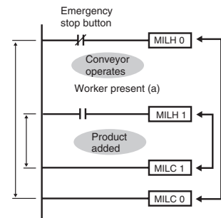
CX-Programmer Screen
