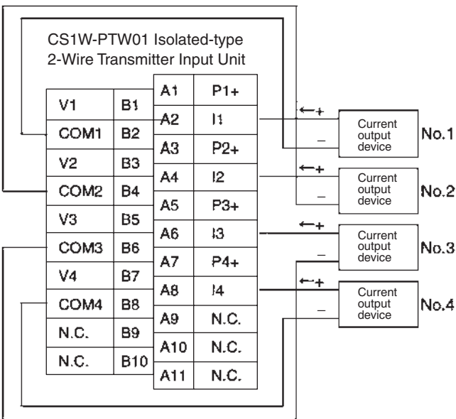
Current input
