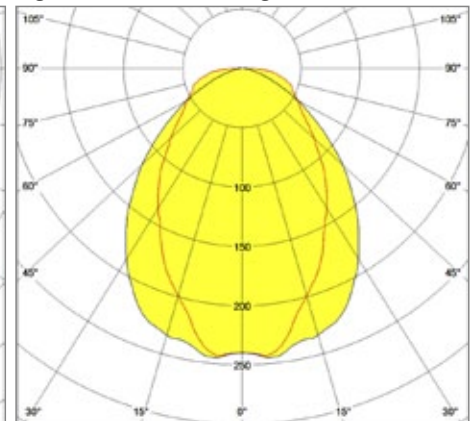
Light distribution Ecolight 26 W
